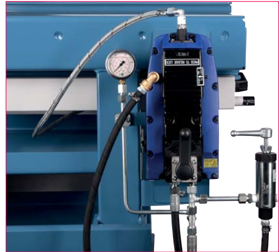
Hydraulic power pack with maintenance unit
